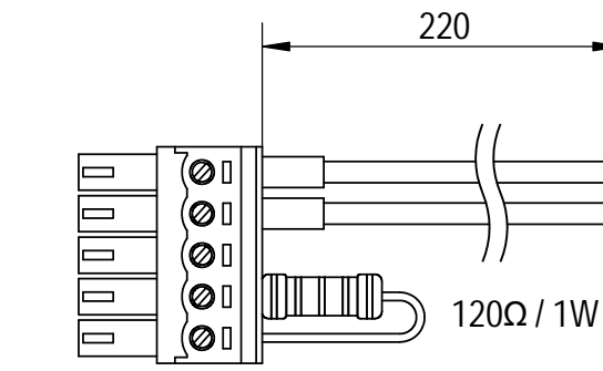
Screw Term. 3.5mm X 5P
